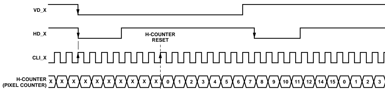
Figure 19. Digital Output Phase Adjustment
