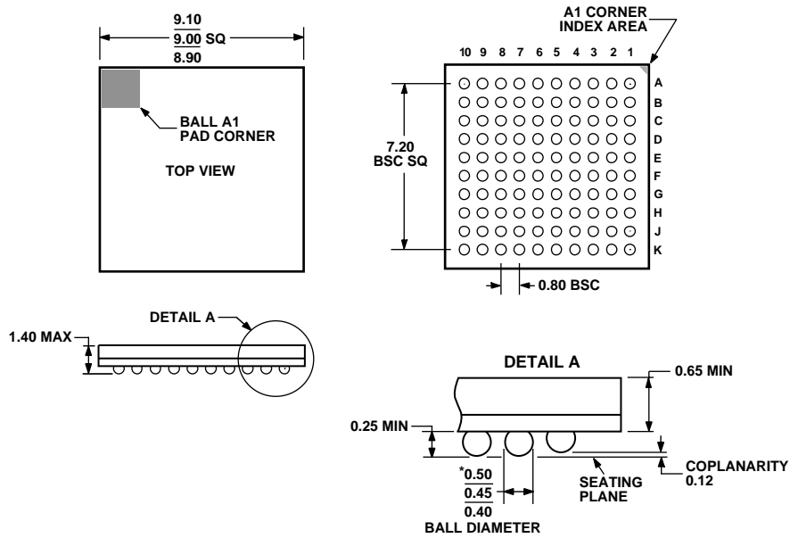
Figure 37. 100-Lead Chip Scale Package Ball Grid Array [CSP_BGA] (BC-100-1) Dimensions shown in millimeters
