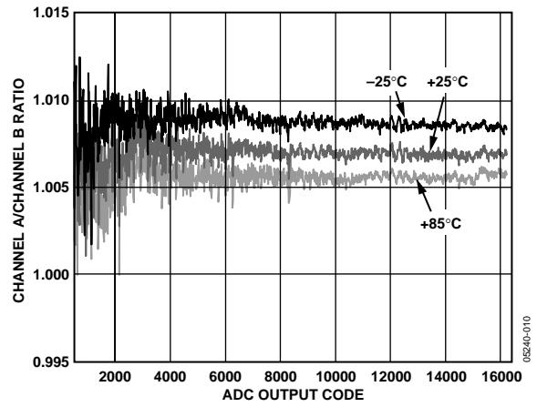
Figure 10. Typical Noncalibrated Channel A/Channel B Ratio
