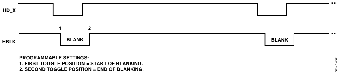
Figure 21. Horizontal Blanking (HBLK) Pulse Placement
