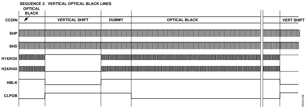
Figure 35. Horizontal Sequences During Vertical Optical Black Pixels
