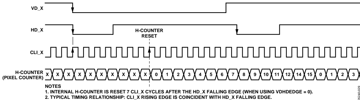
Figure 26. H-Counter Synchronization
