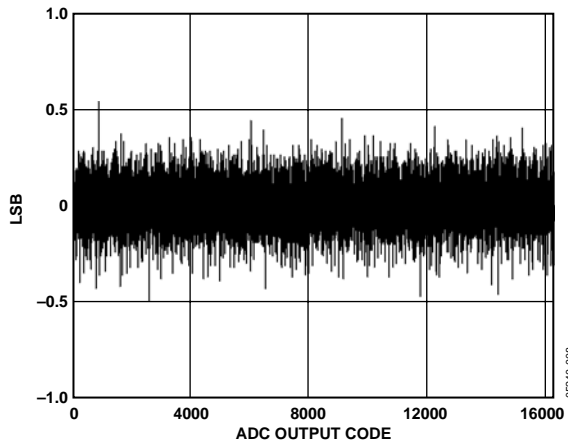
Figure 8. Typical DNL for Channel A and Channel B
