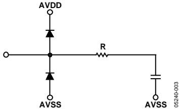
Figure 3. CCDIN_X
