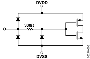
Figure 6. Digital Inputs
