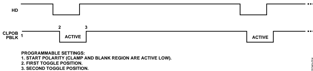
Figure 22. Clamp and Preblank Pulse Placement
