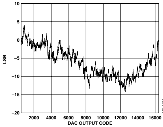
Figure 9. Typical INL Performance for Channel A and Channel B
